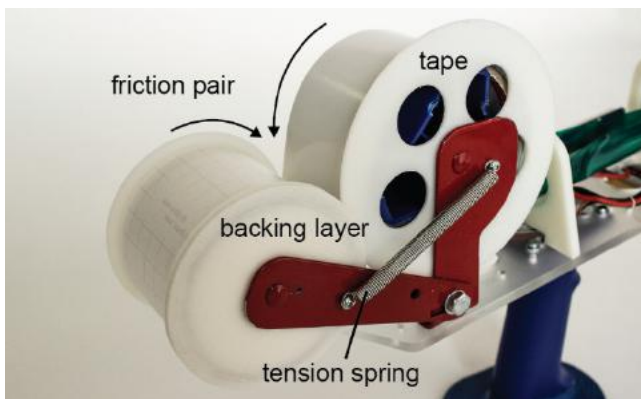
Figure 9: A second spool gathers the tape’s backing layer
