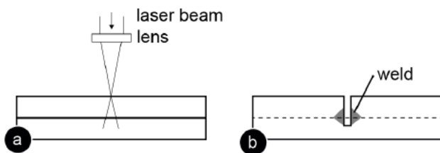
Figure 5: Welding two sheets of acrylic: (a) the laser cuts through the top layer and into 30% of bottom layer, (b) the heat along the laser path welds both layers.
