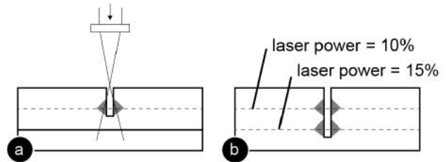
Figure 13: We increase the laser power as we move away from the focal point of the laser.
