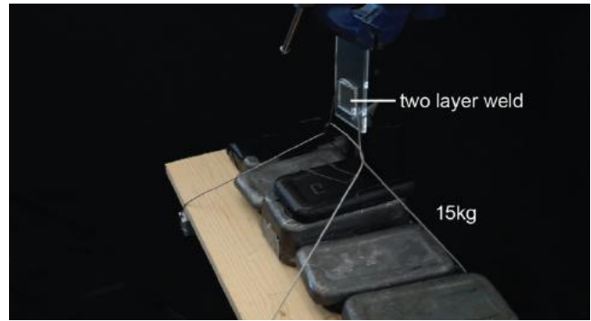
Figure 16: A weld holds more than 15kg of weight.
