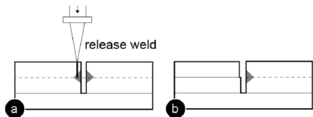
Figure 7: Releasing a weld: (a) creating a new cut in very close proximity, (b) the material evaporates and releases the weld.
