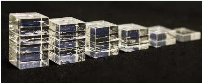
Figure 14: Calibration pattern to determine laser power for welding up to six layers of acrylic.
