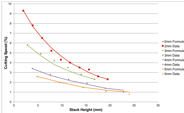
Figure 15: Measured data points and predicted data points based on the laser welding formula.
