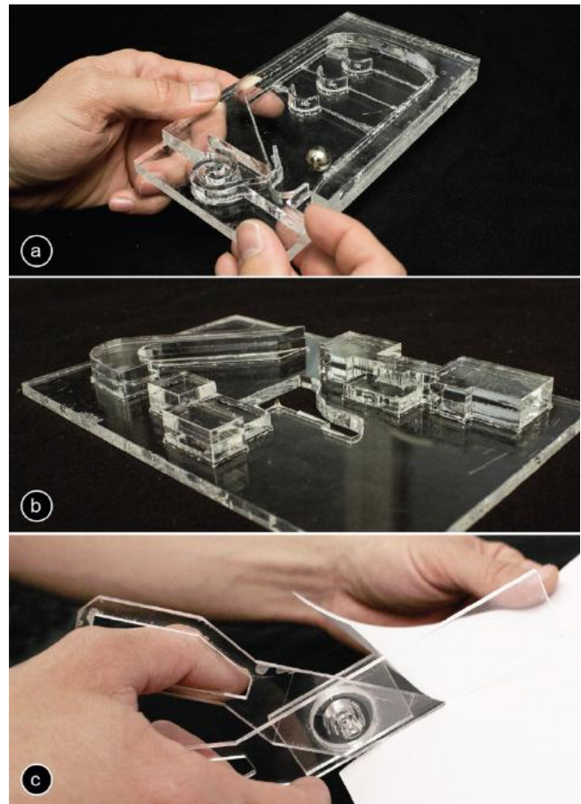
Figure 1: LaserStacker produces laser cut objects consisting of multiple layers of acrylic without requiring manual assembly: It assembles the object by not only cutting with the laser, but also welding, and healing the cut. Three example objects: (a) a pinball table with spring (10 min), (b) an architectural model of our university campus (7 min), and (c) a simple but functional pair of scissors (3 min).
