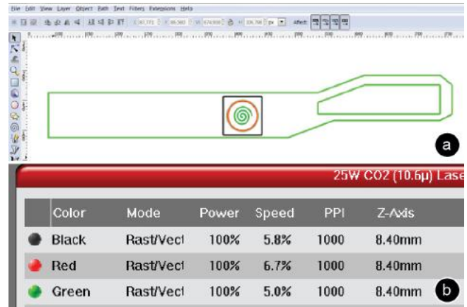
Figure 11: LaserStacker exports (a) an .svg file with 2D paths, and (b) a laser settings file with the power/speed settings, here we already loaded it into the laser cutter's control panel.
