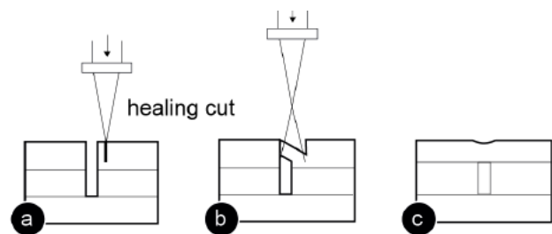
Figure 6: Healing a cut: (a) creating a new cut in close proximity, (b) defocusing the laser and melting the piece to (c) create a strong side-by-side weld.
